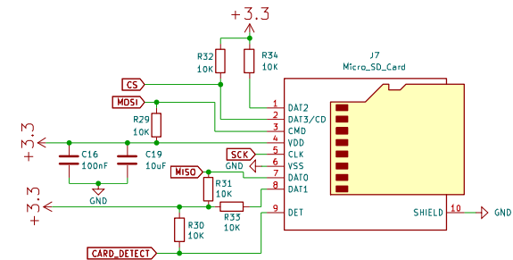
SD-CARD
