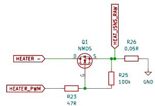
HEATER MOSFET AND CURRENT SENSE
