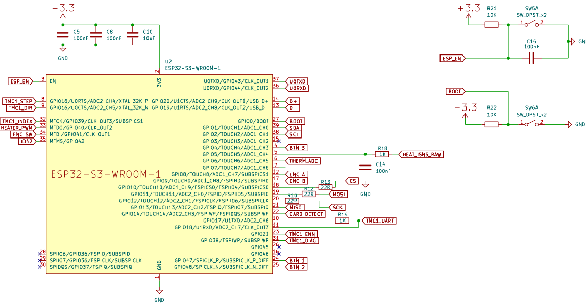
ESP32-S3-WROOM-01 - DECOUPLING - RESET AND BOOT BUTTONS
