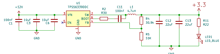
3V3 LINE - TPS56339DDC
